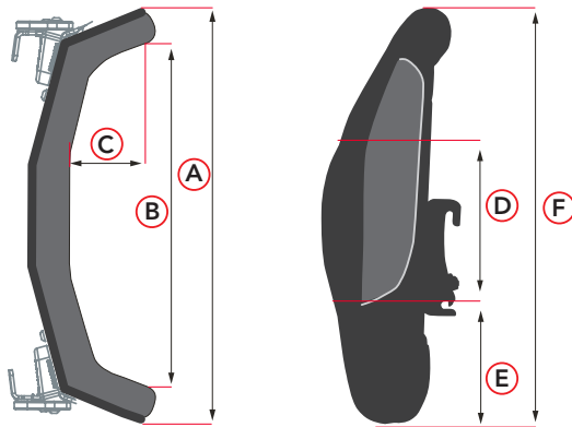
BACK DIMENSIONS – INCHES (CM)
